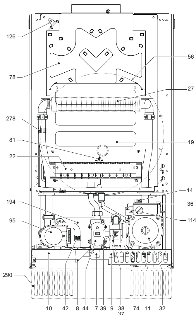
fig. 13 - General view FL 24 MCA
