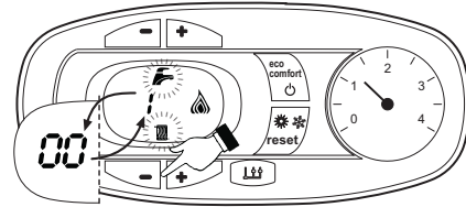
fig. 9 - Mode TEST (puissance chauffage = 100%)
