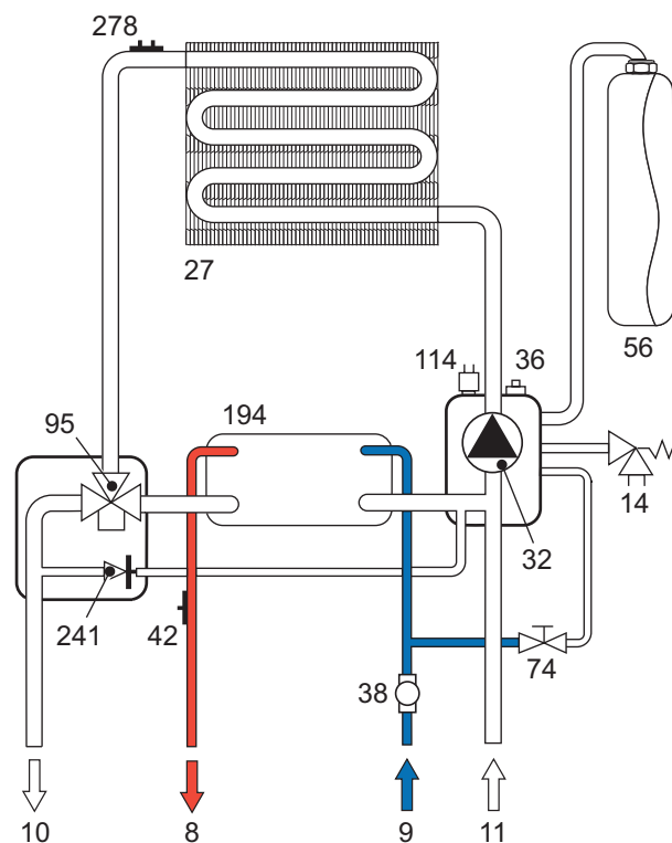
fig. 15 - DHW Circuit
