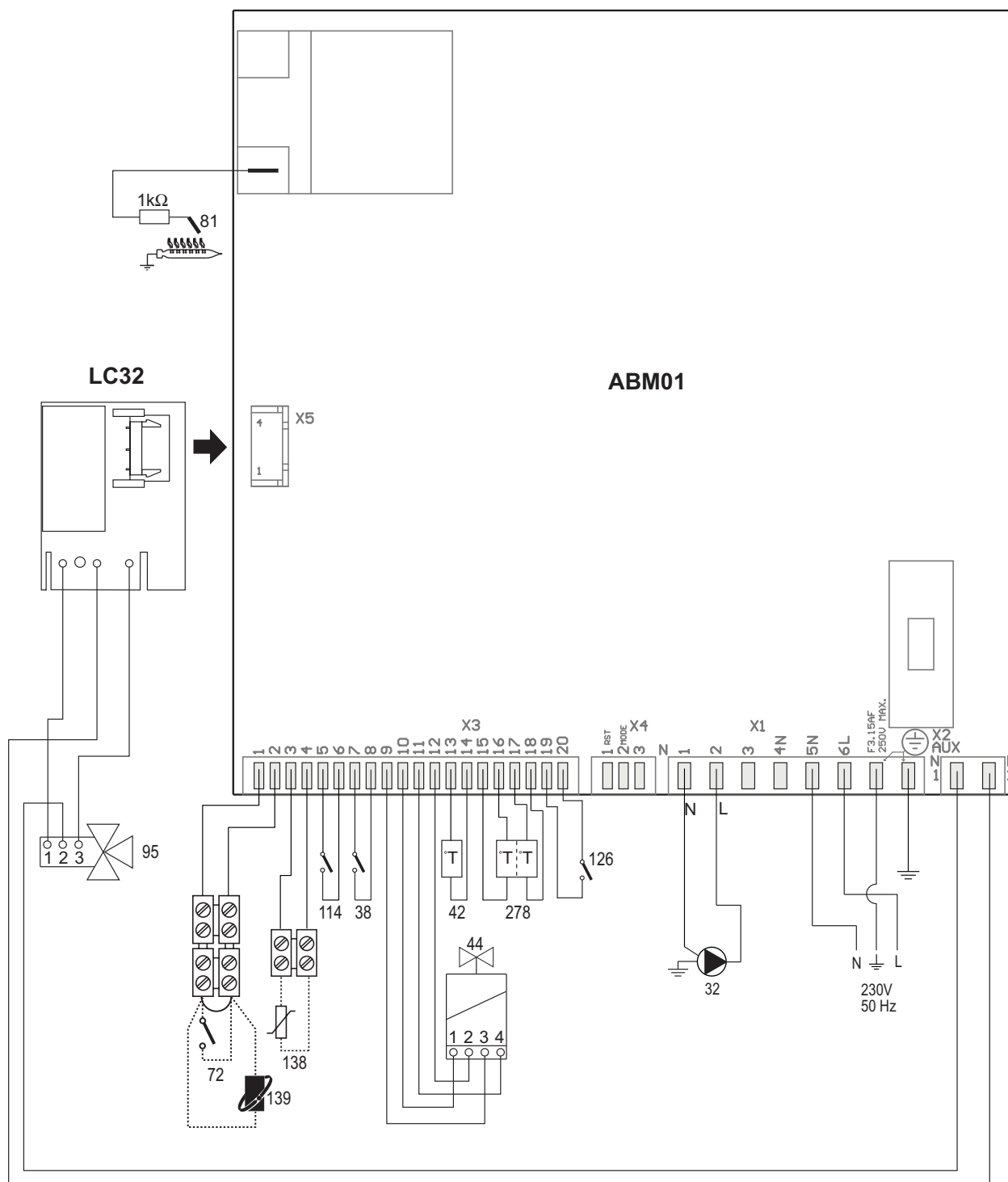
fig. 16 - Electrical circuit
