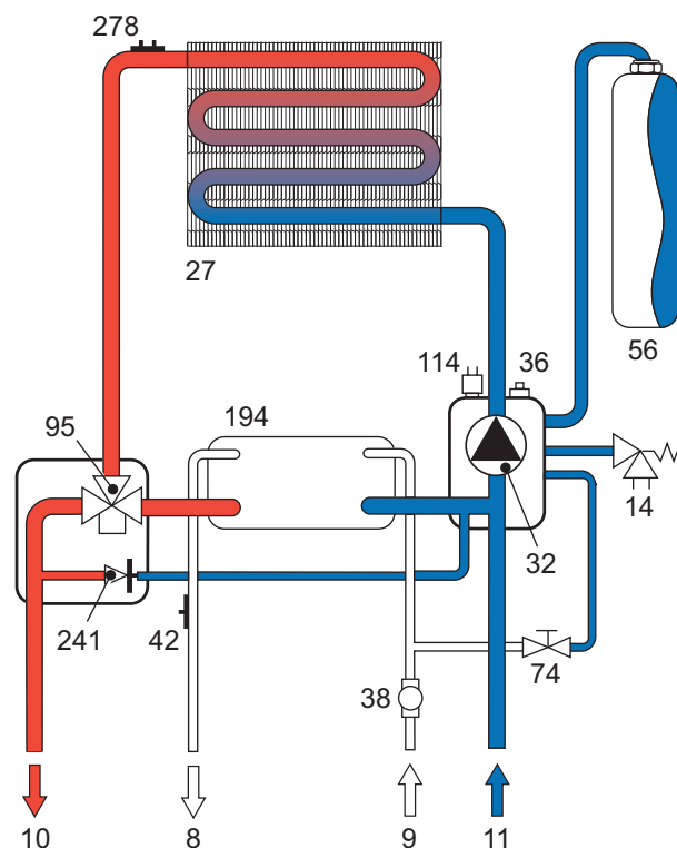
fig. 14 - Heating Circuit
