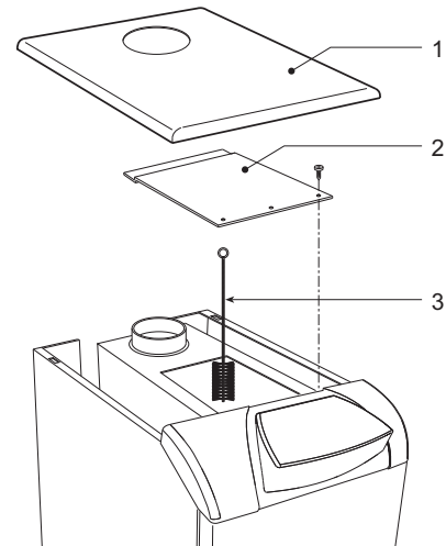
fig. 19 - Boiler cleaning
