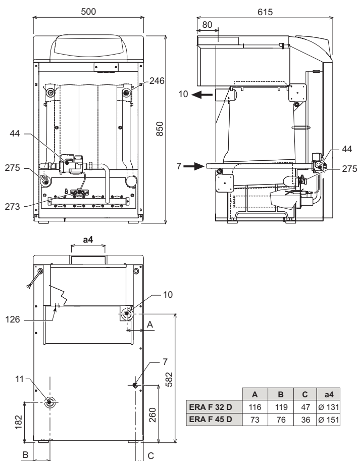
fig. 23 - Dimensions and connections model ERA F 32 D and ERA F 45 D
