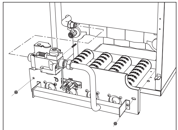
fig. 20 - Removing the burners
