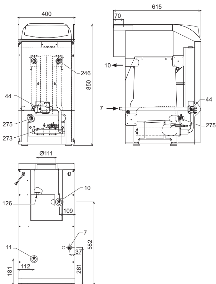
fig. 22 - Dimensions and connections model ERA F 23 D
