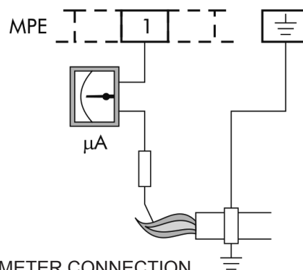
MICROAMPEREMETER CONNECTION
