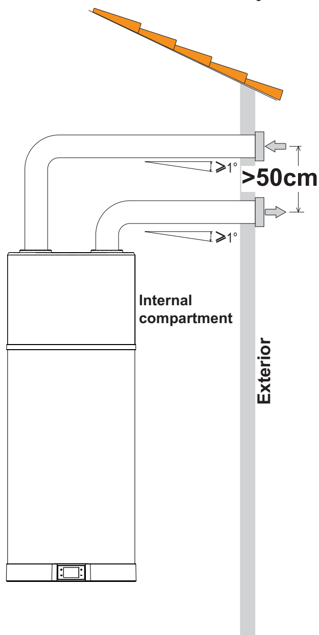
fig. 12 - Example of air outlet connection
