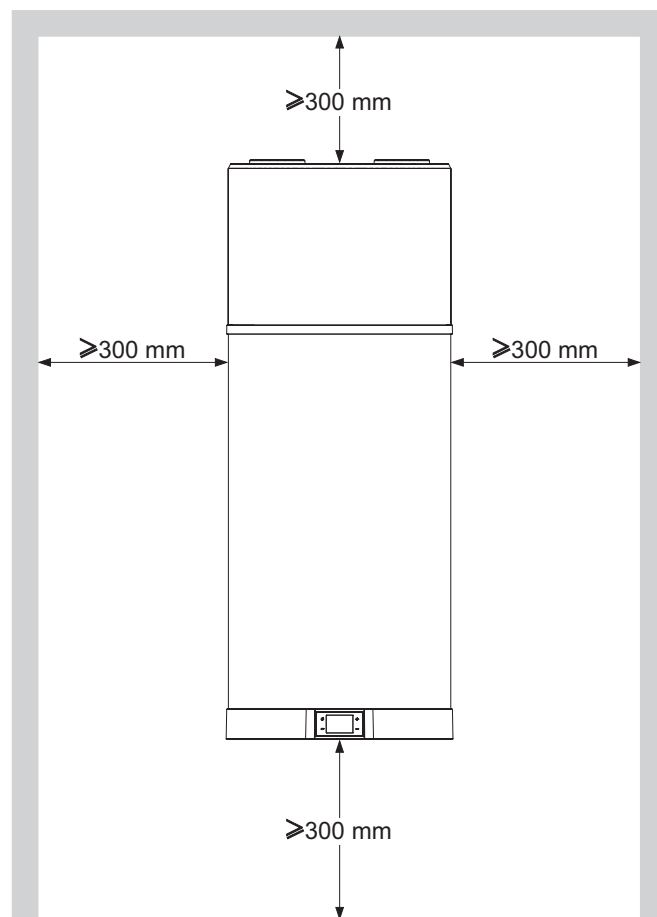
fig. 9 - Minimum spaces
