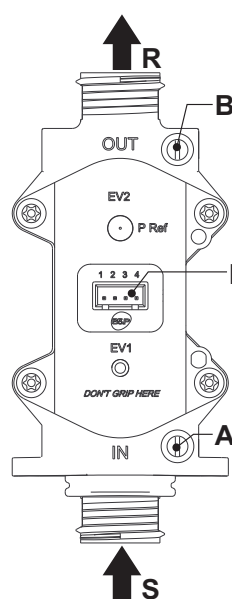
fig. 11 - Gas valve
