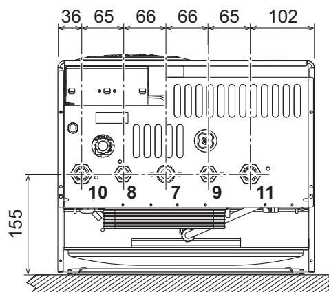
fig. 18- Bottom view - FL D L N C24 and C30
