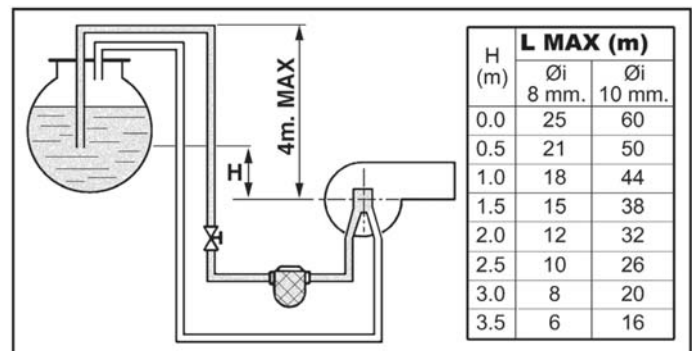
fig.20 - Siphon feed
