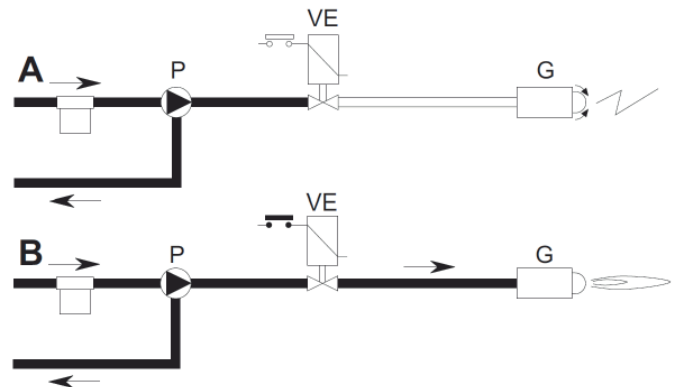
fig.30 - Starting
