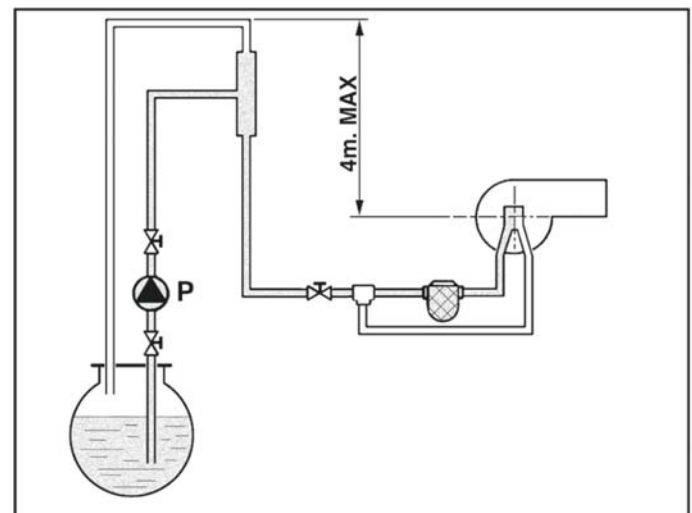
fig.21 - Ring feed
