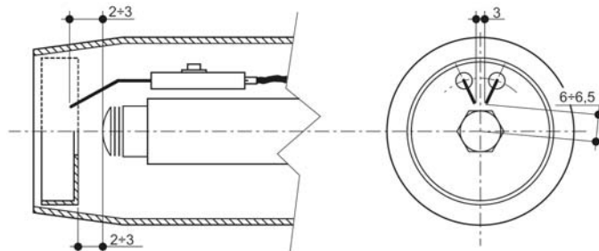
fig.29 - Position of electrodes - baffle
