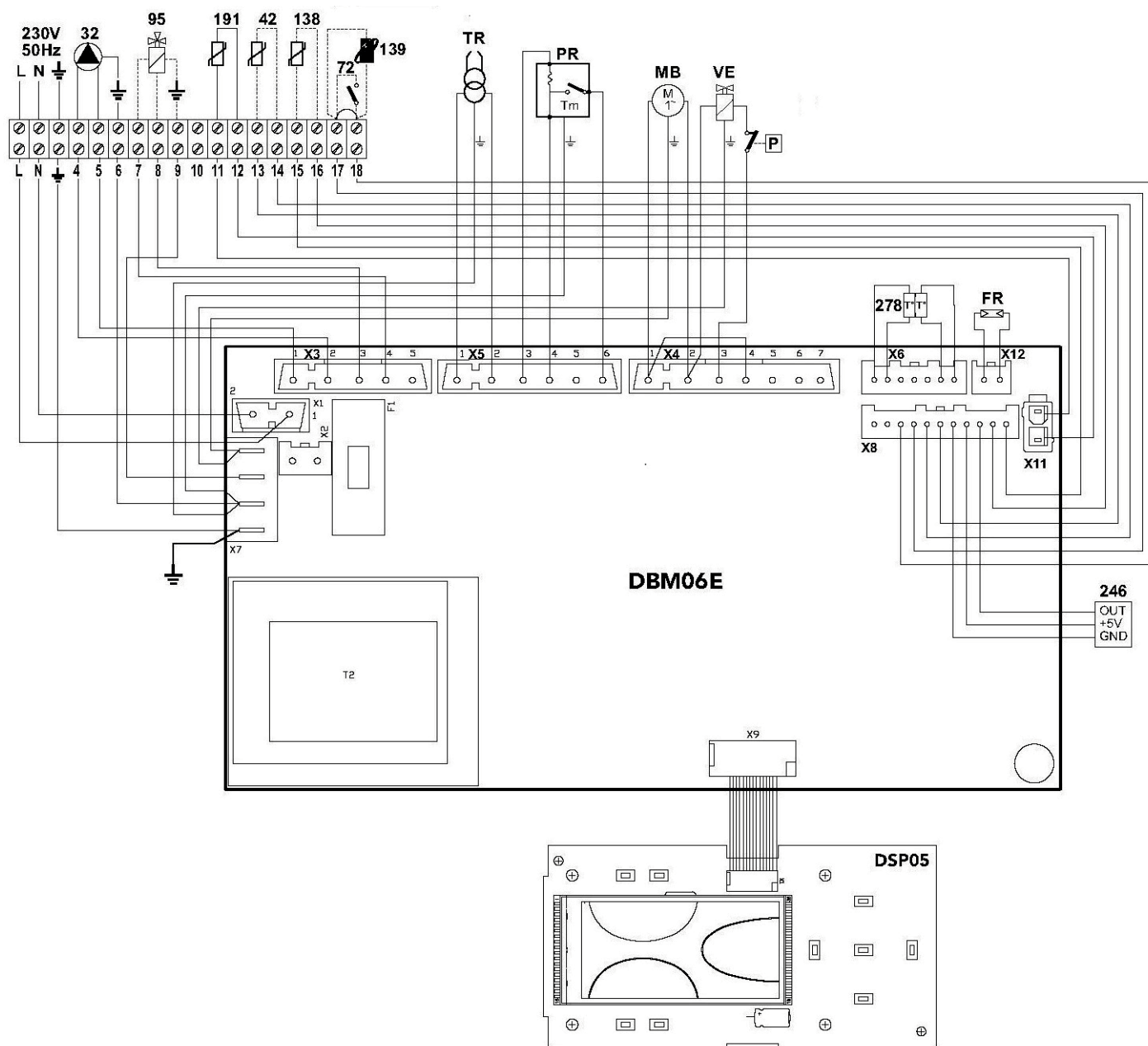
fig.42 - Wiring diagram
