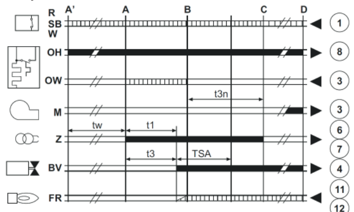
fig.31 - Unit cycle
