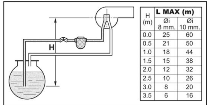
fig.19 - Suction feed
