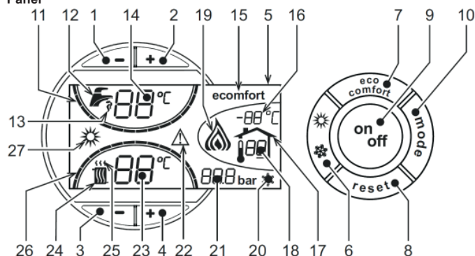
fig.1 – Control panel
