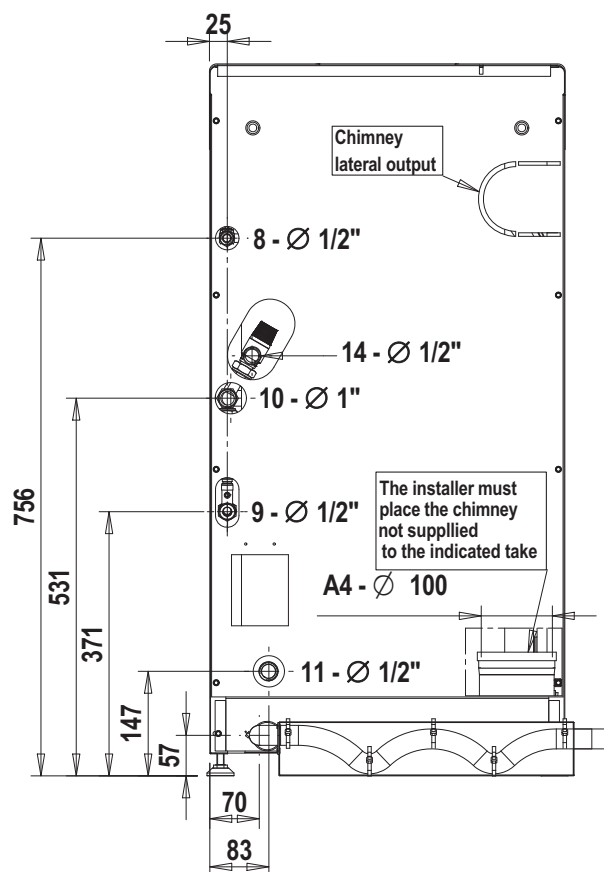
fig.38 - Rear view
