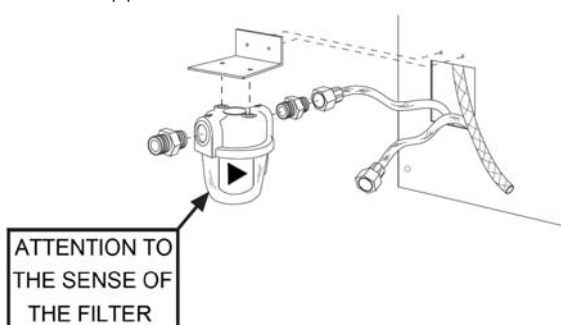
fig.18 - Fuel filter installation
