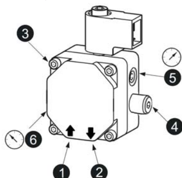
fig.26 - Pump DANFOSS
