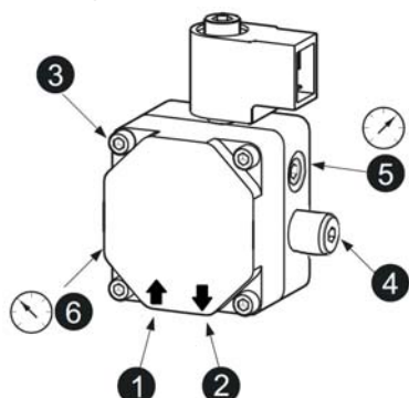
fig.26 - Bomba DANFOSS
