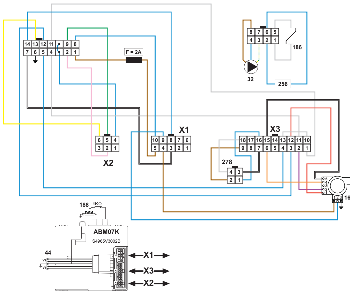
fig. 121- Intermediate module wiring diagram
