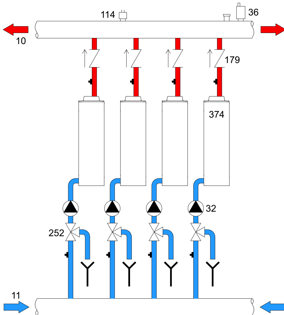
fig. 115- Hydraulic circuit
