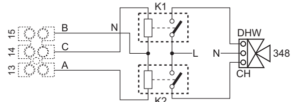
fig. 117- Connection of the 3-way valve with 3 wires
