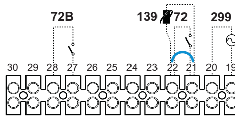
fig. 101- Par. P01 connections diagram P.01
