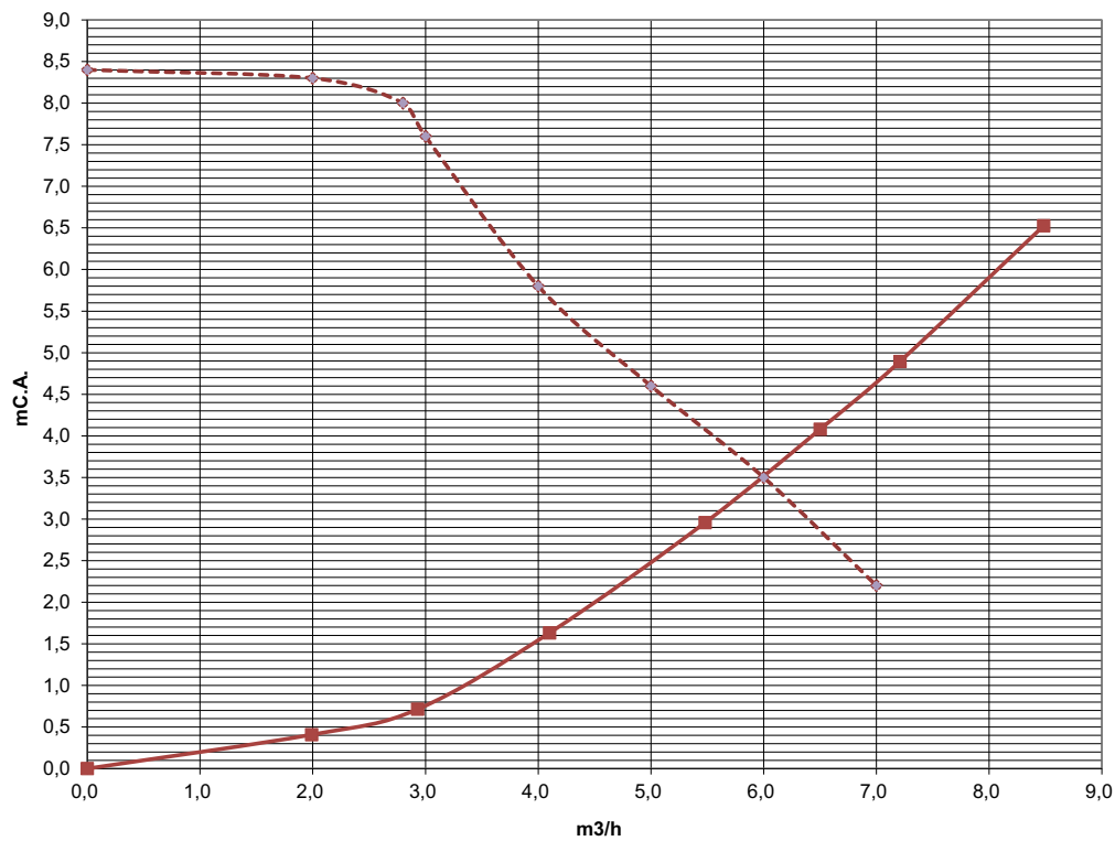
Circulating pump head / pressure losses TITAN 225
