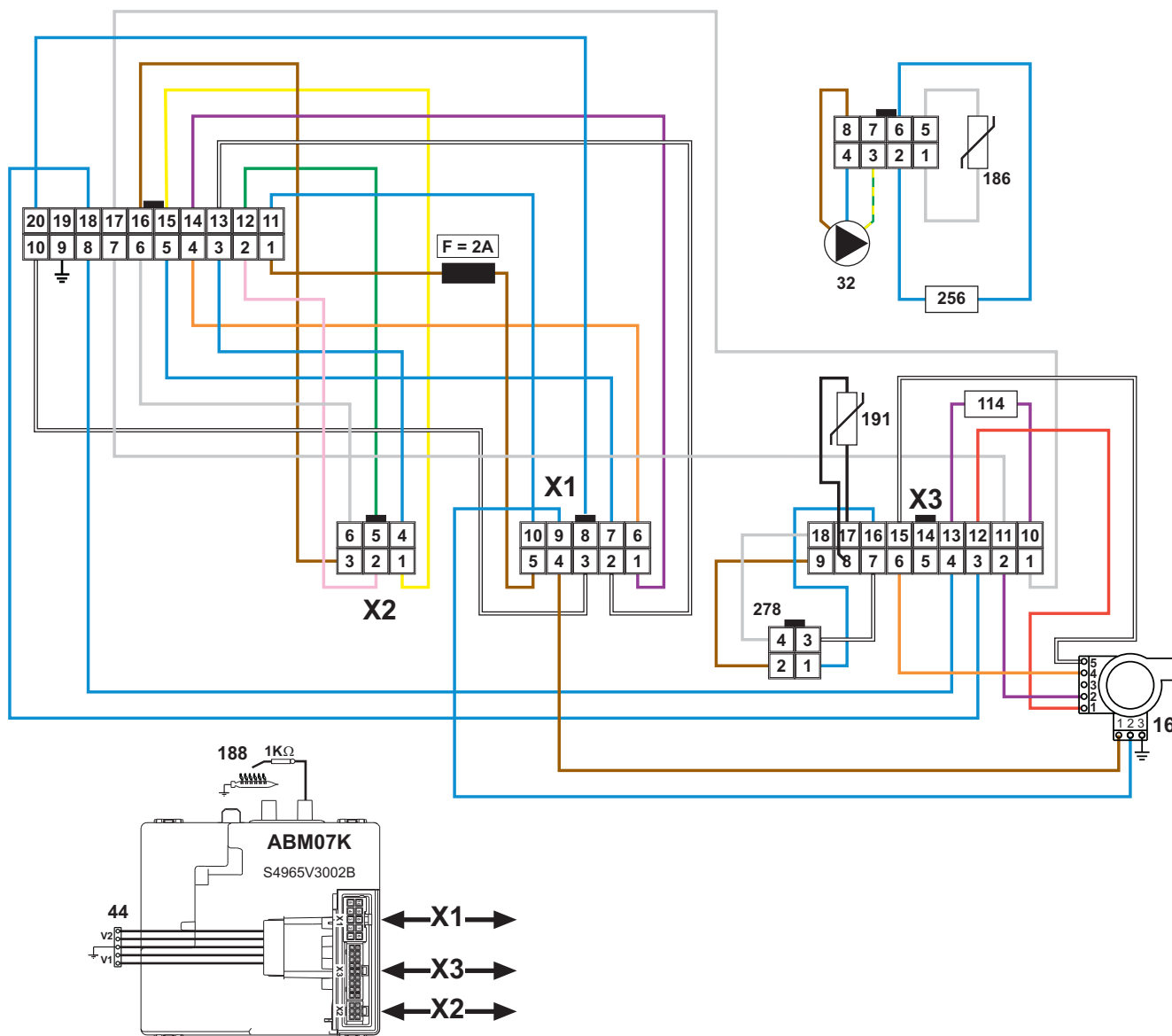
fig. 120- First module wiring diagram
