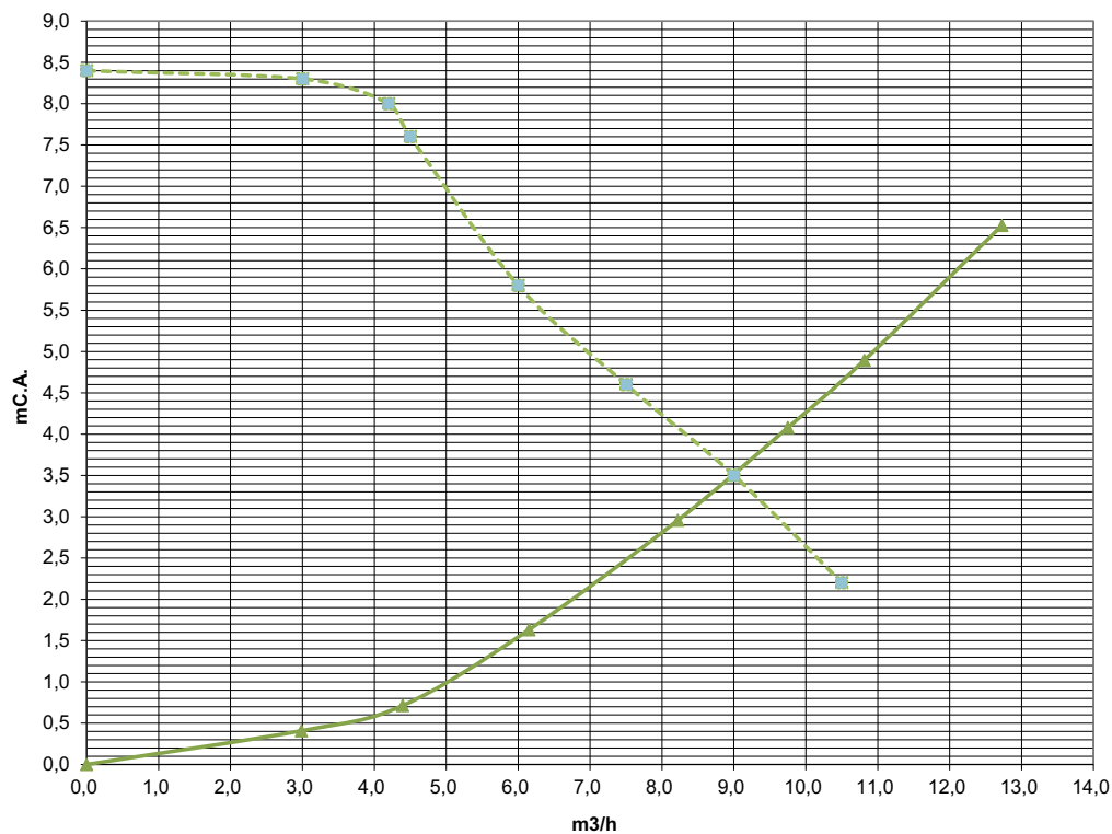
Circulating pump head / pressure losses TITAN 225
