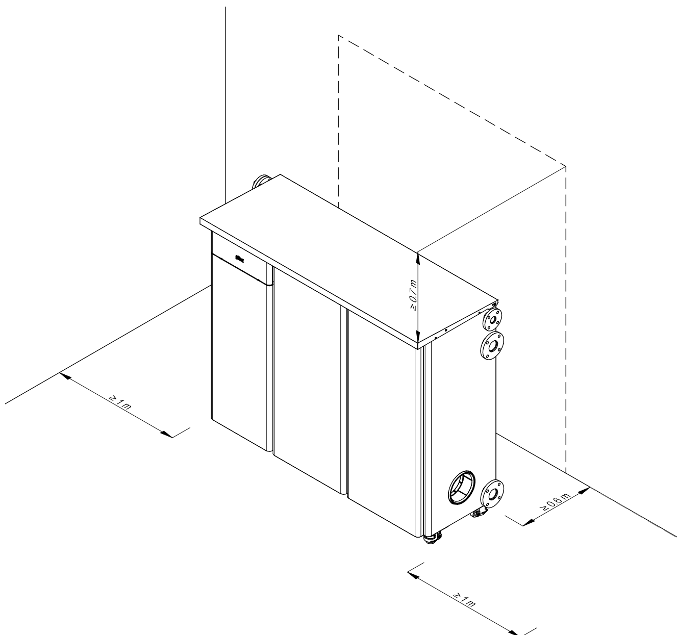
fig. 37- Positioning with distances to be respected
