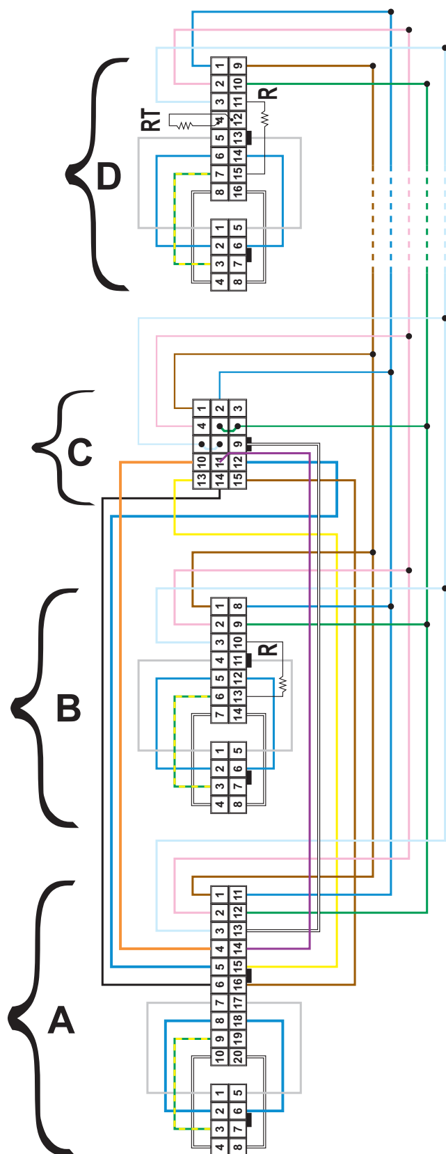
fig. 123- Module connection cable wiring diagram
