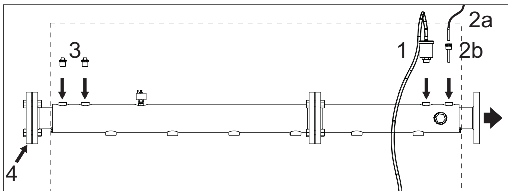
fig. 41- Right side delivery
