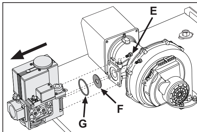
fig. 61 - Modello CLOVER 220
