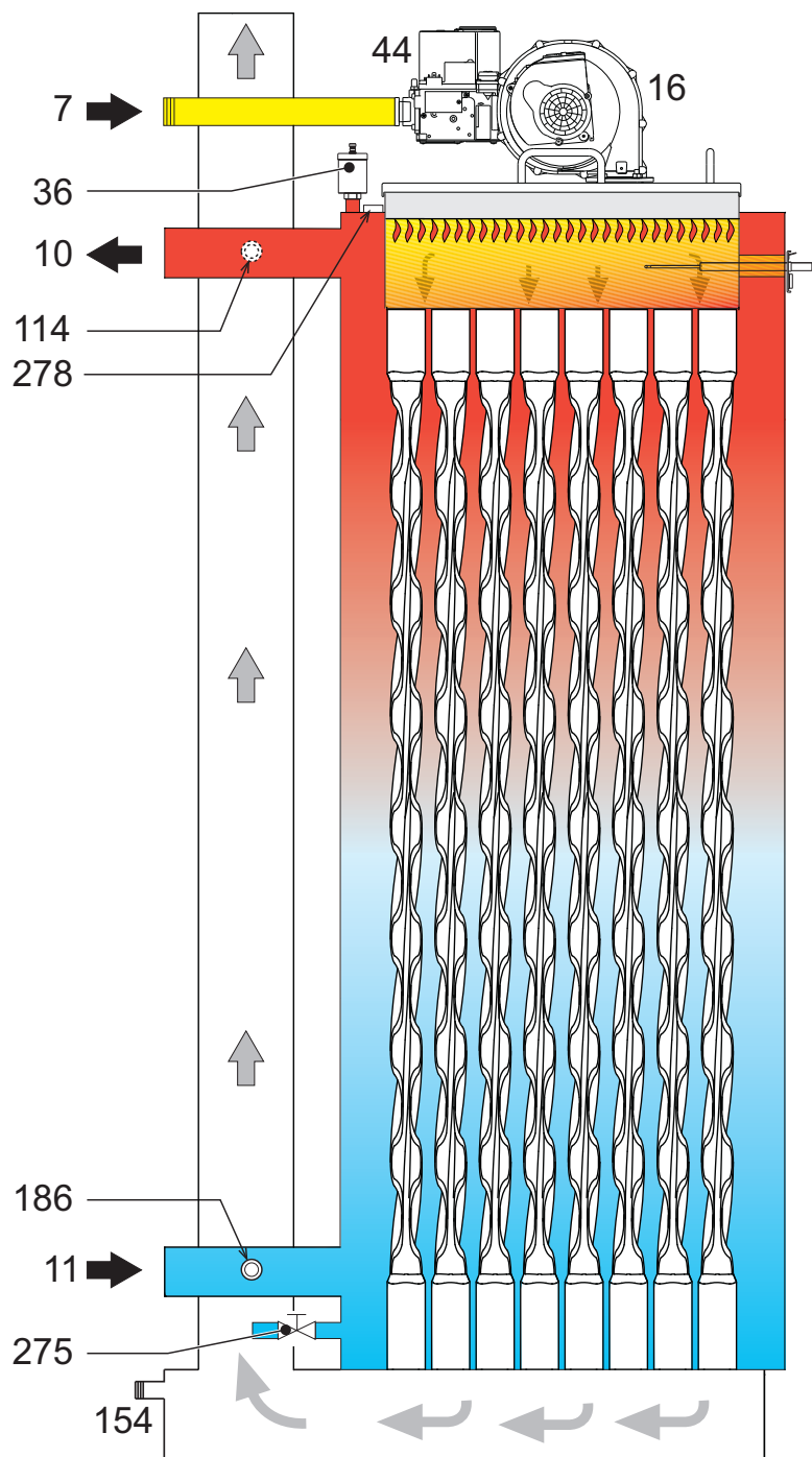
fig. 86- Hydraulic circuit
