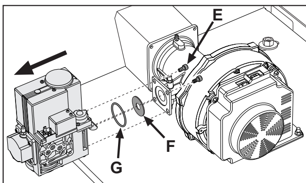
fig. 62- Model CLOVER 320
