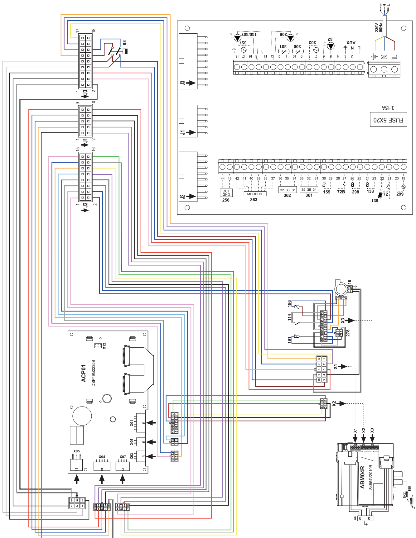
fig. 93- Wiring diagram CLOVER 125 and 160
